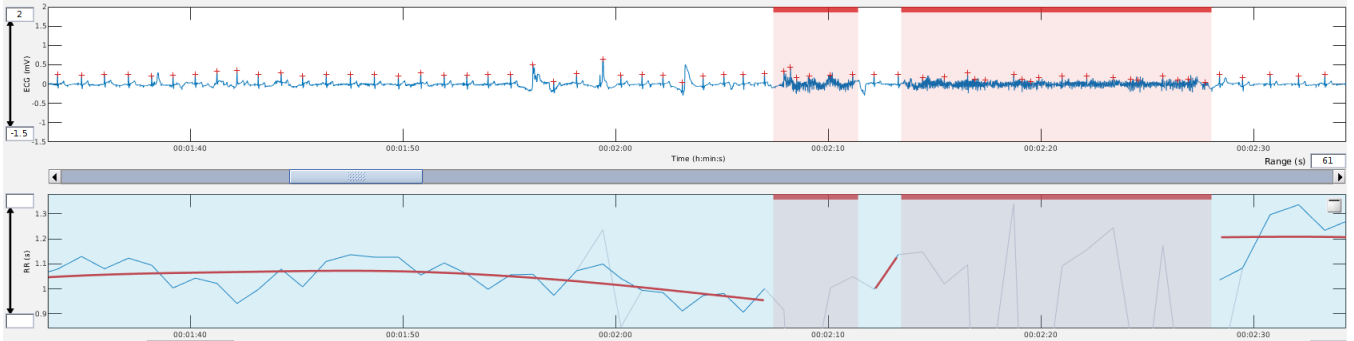
Fig. 4: The raw ECG signal (top). Noisy segments were marked (red background) and removed from the analysis. R-R intervals were extracted from the QRS signal (bottom).
